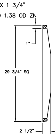
GRATE SECTION
