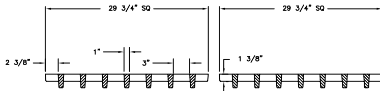
GRATE SECTION
