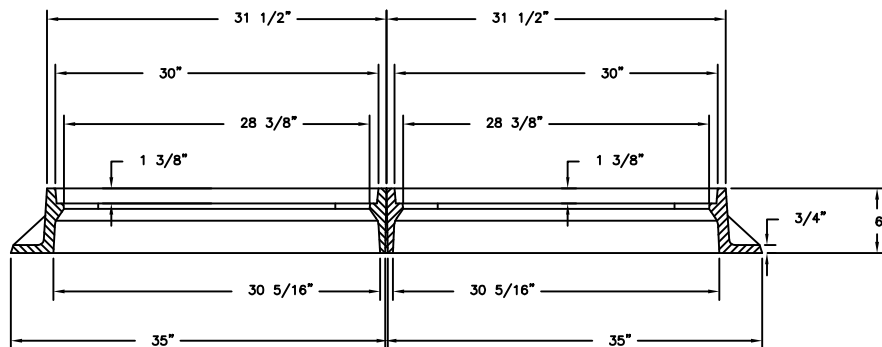
FRAME SECTION
