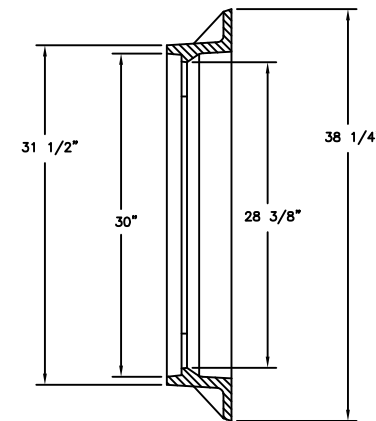
FRAME SECTION
